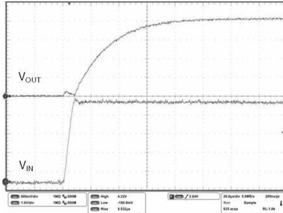
Figure 30. Startup transient
