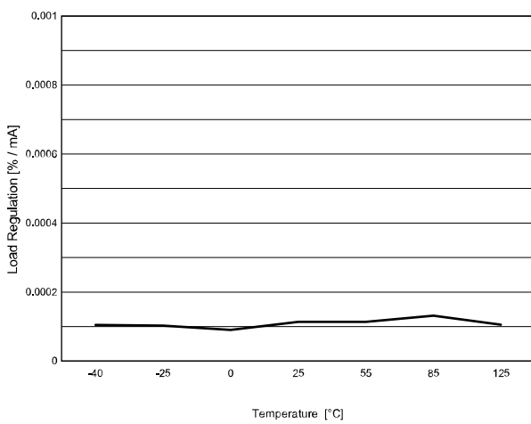
Figure 10. Load regulation vs. temperature ( V_{IN} = 6 V, V_{OUT} = 5 V, I_{OUT} = 10 to 1200 mA)
