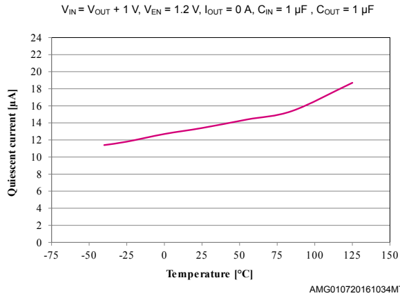
Figure 8. Quiescent current vs. temperature ( I_{OUT} = 0 \text{ mA} )
