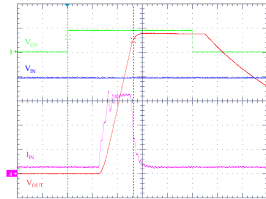
Figure 27. Inrush current
