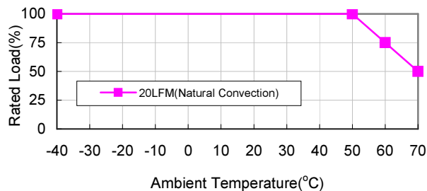
Derating curve:
