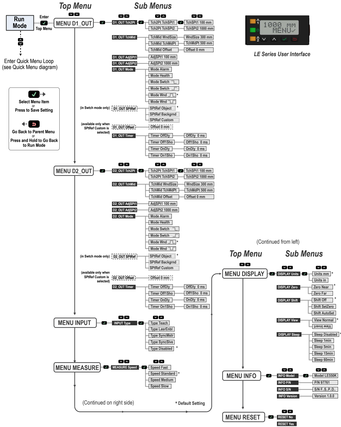
Figure 14. LE550 Sensor Menu Map
