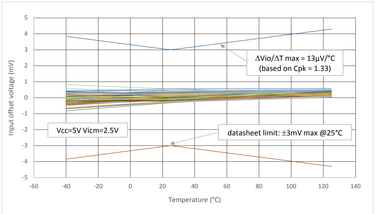
Figure 13. LMV358YPT Input offset voltage vs. temperature at 5 V supply voltage
