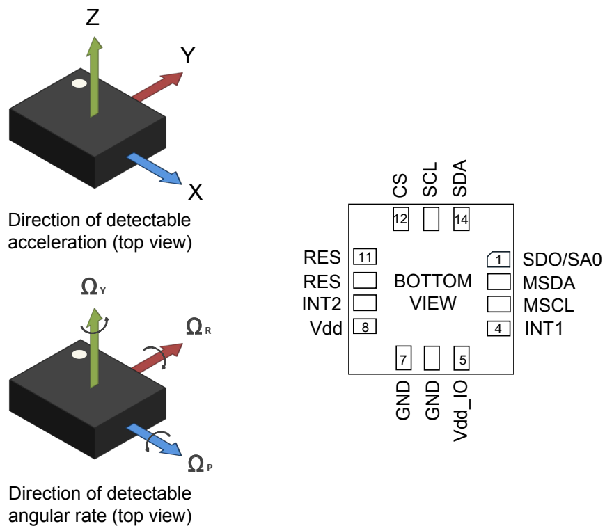
Figure 2. Pin connections
