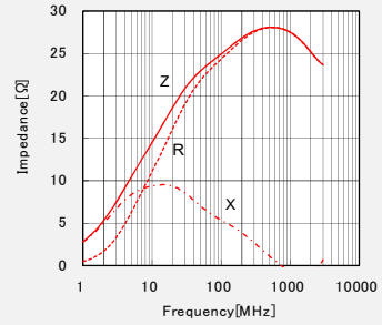
LSMCC201208T250NG
