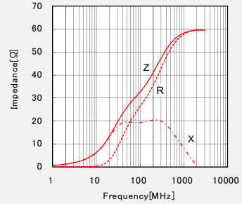
LSMCA201208T330RG
