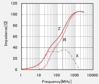
LSMCA451611T560NG
