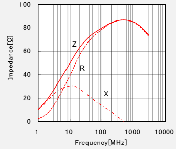
LSMCC321611T800RG
