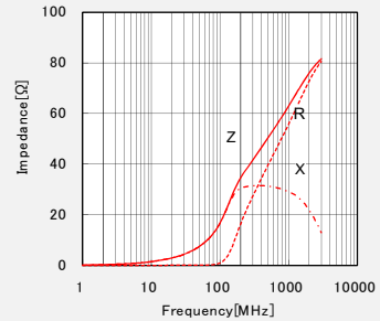
LSMCG321611T160NG
