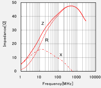
LSMCC201208T420RG
