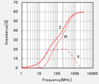
LSMCA201208T330RG
