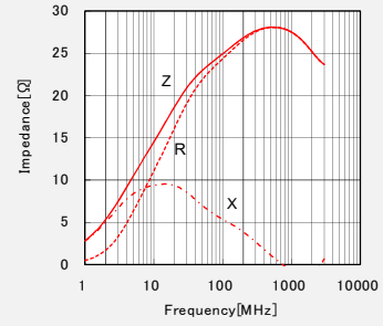
LSMCC201208T250NG
