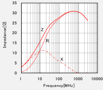
LSMCC160808T280NG
