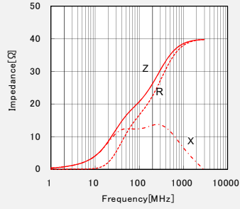
LSMCA201208T210NG
