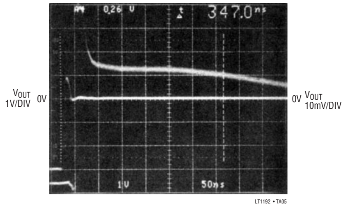
SETTLING TIME TO 10mV , A_V = 2 SUPPLY BYPASS CAPACITORS = 0.1\mu F
