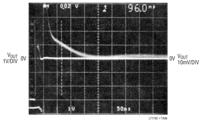
SETTLING TIME TO 10mV , A_V = 2 SUPPLY BYPASS CAPACITORS = 0.1\mu F + 4.7\mu F TANTALUM
