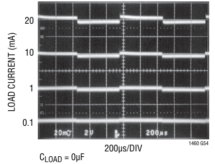
LT1460S3-10V Transient Response
