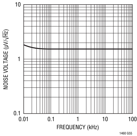
LT1460S3-10V Output Voltage Noise Spectrum
