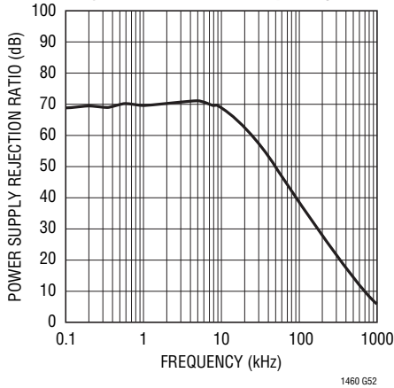
LT1460S3-10V Power Supply Rejection Ratio vs Frequency
