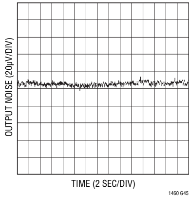
LT1460S3-2.5V Output Noise 0.1Hz to 10Hz
