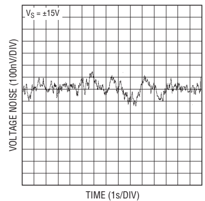
0.1Hz to 10Hz Voltage Noise
