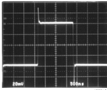
±15V Small-Signal Response
