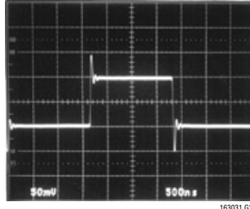
5V Small-Signal Response
