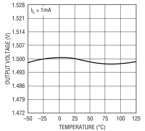
LT1761-1.5 Output Voltage
