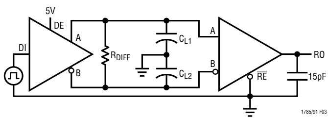
Figure 3. Driver/Receiver Timing Test Circuit
