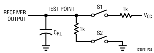
Figure 2. Receiver Timing Test Load
