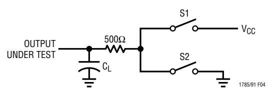
Figure 4. Driver Timing Test Load
