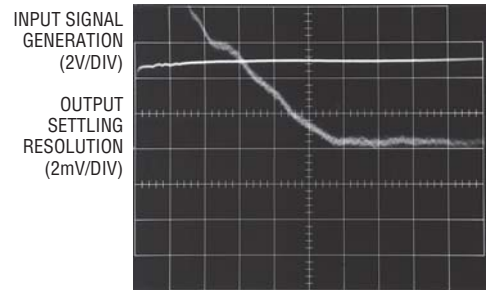
0.01% Settling Time
