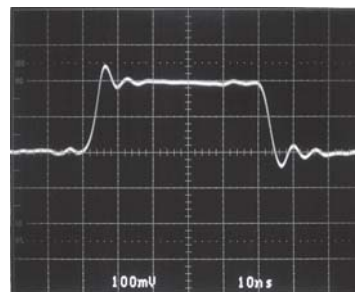
10ns/DIV 1809 G42 V_S = \pm 5V A_V = +1 R_L = 1k
