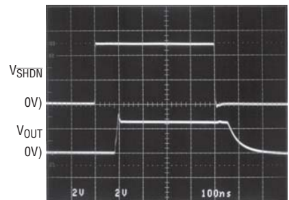
100ns/DIV 1809 G44 V_S = 5V, 0V A_V = +2 R_L = 100\Omega
