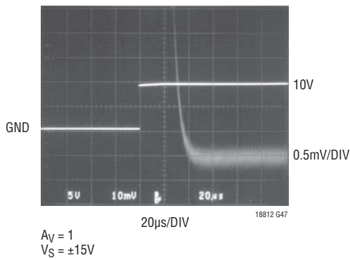
Settling Time/Output Step 0.01%
