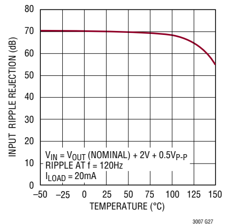
Input Ripple Rejection
