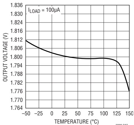
Output Voltage LT3008-1.8
