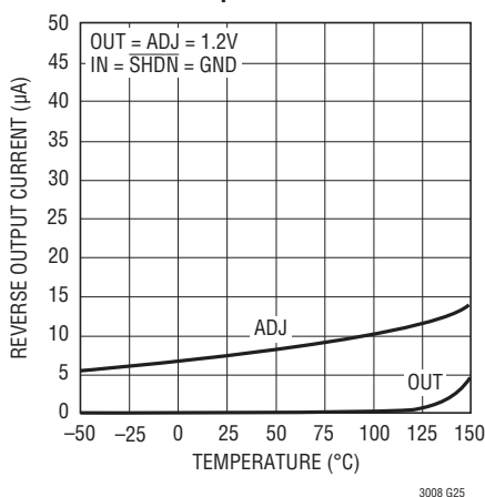
Reverse-Output Current
