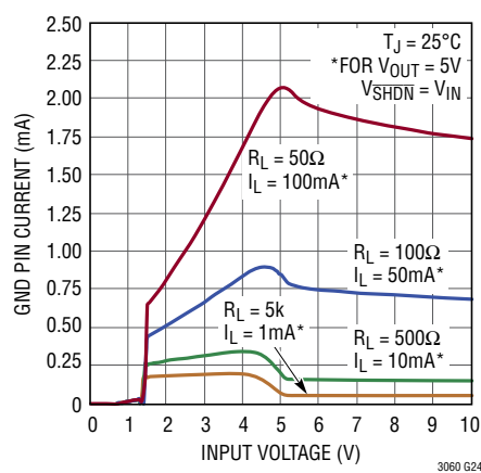
LT3060-5 GND Pin Current
