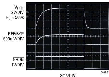
SHDN Transient Response C_{REF/BYP} = 10\text{nF}
