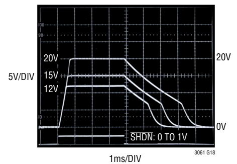
Output Discharge vs V_{OUT} C_{REF}/\text{BYP} = 0
