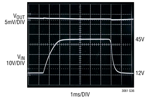
Transient Response, V_{OUT} = 5\text{V} Load Dump, V_{IN} = 12\text{V TO } 45\text{V}
