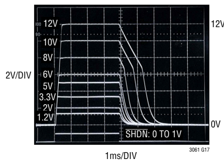
Output Discharge vs V_{OUT} C_{REF}/\text{BYP} = 0
