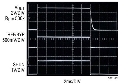
SHDN Transient Response C_{REF/BYP} = 0
