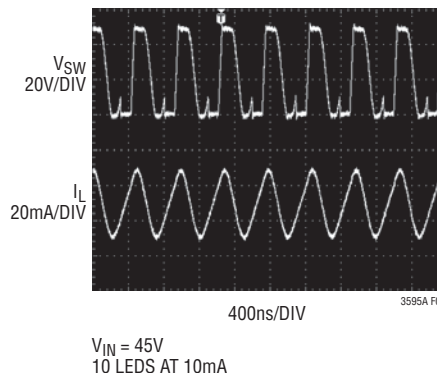
Figure 1. Switching Waveforms
