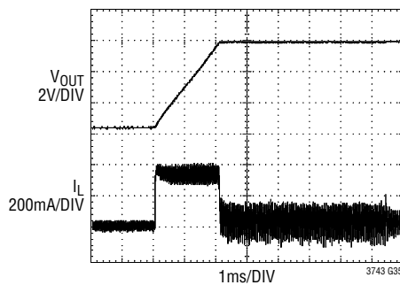
Common Mode Lockout (V IN = 7V)
