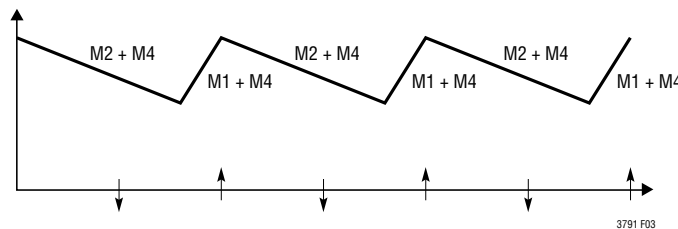
Figure 3. Buck Operation ( V_{IN} > V_{OUT} )
