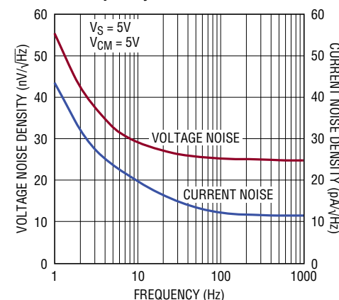
Over-The-Top Noise Density vs Frequency
