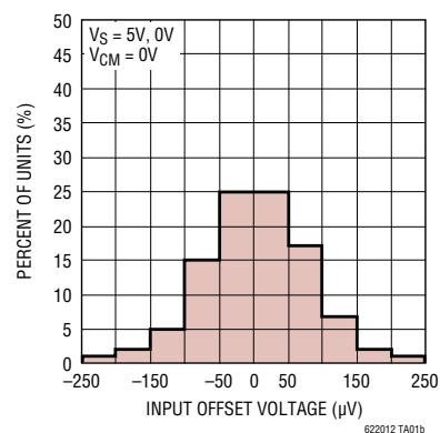
V_{\text{OS}} Distribution, V_{\text{CM}} = 0\text{V} (S8, PNP Stage)
