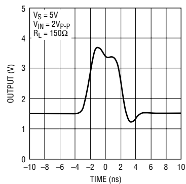
Fast Large-Signal Transient Response
