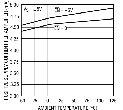
Positive Supply Current per Amplifier vs Temperature
