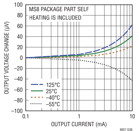
5V Load Regulation (Sourcing)
