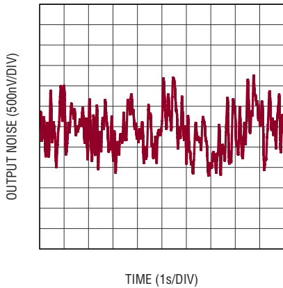
5V Low Frequency 0.1Hz to 10Hz Noise
