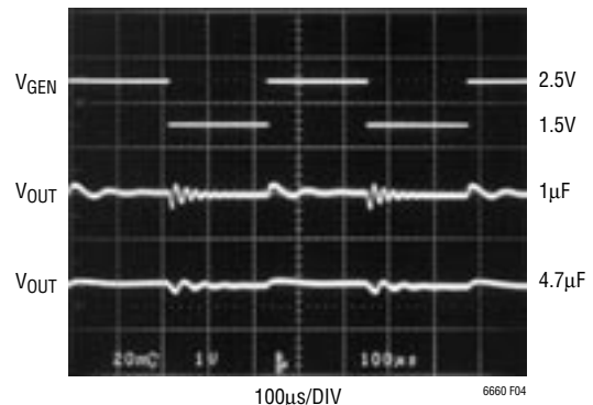
Figure 4. I_{OUT} = 1mA
