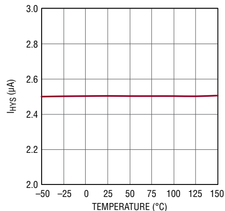
EN/UVLO Hysteresis Current
