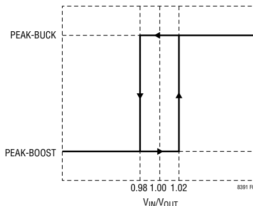
Figure 2. Current Mode vs V_{IN}/V_{OUT} Ratio
