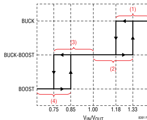
Figure 3. Operation Region vs V_{IN}/V_{OUT} Ratio
