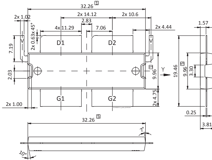
Package PG-HB2SOF-6-1
