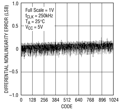
Differential Nonlinearity
