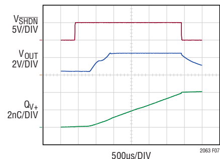
Figure 7. LTC2063 Charge Loss Due to Enabling and Disabling via \overline{\text{SHDN}} Pin
