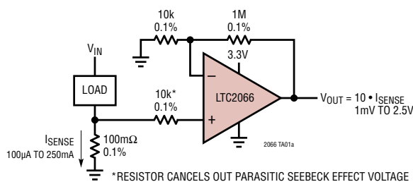
Precision Micropower Low Side Current Sense
