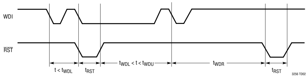
Watchdog Timing
