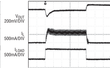
Load Step
