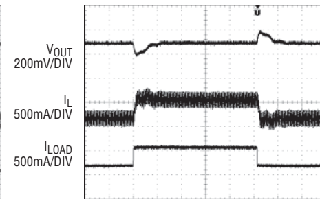
Load Step
