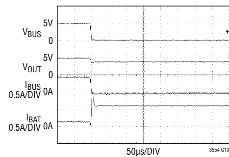
V_{\text{BUS}} Disconnect Waveform
