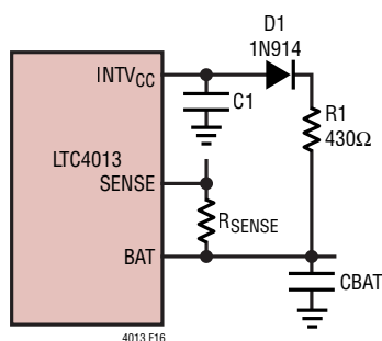
Figure 15. SENSE Precharge
