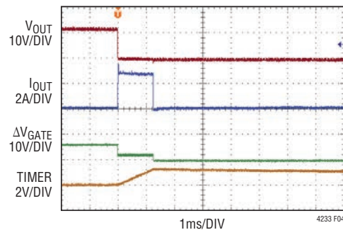
Figure 4. Short-Circuit Waveform
