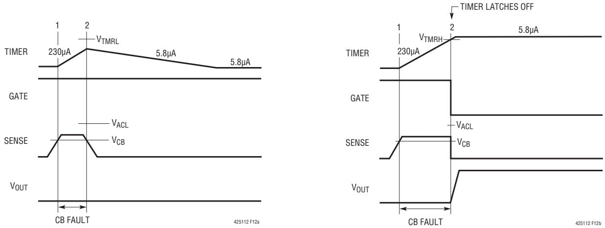
(12a) Momentary Circuit-Breaker Fault
