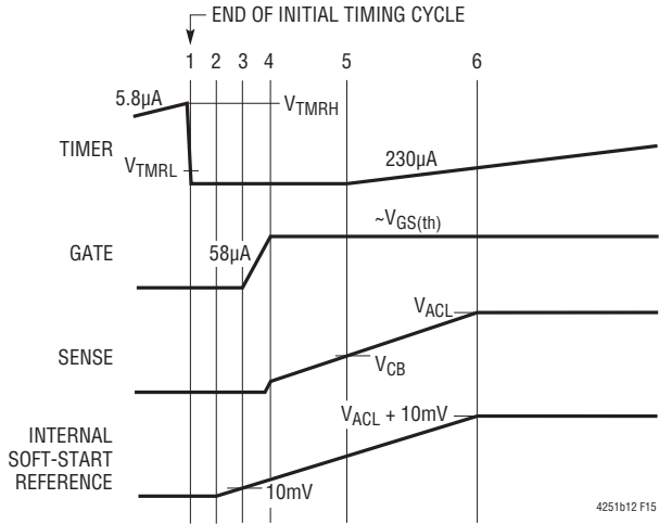
Figure 15. Internal Soft-Start Timing (All Waveforms are Referenced to V_{\text{EE}} )
