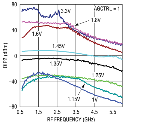
Output IP2 vs RF Frequency and V CTRL
