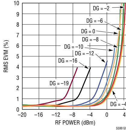
RMS EVM vs RF Output Power with 1Ms/s 16-QAM Signal
